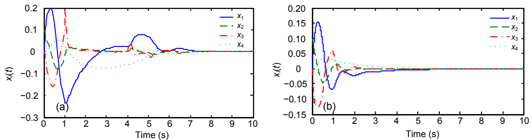
Fig. 3 Power system responses of ADP (a) and IAFOC (b) in case 1
